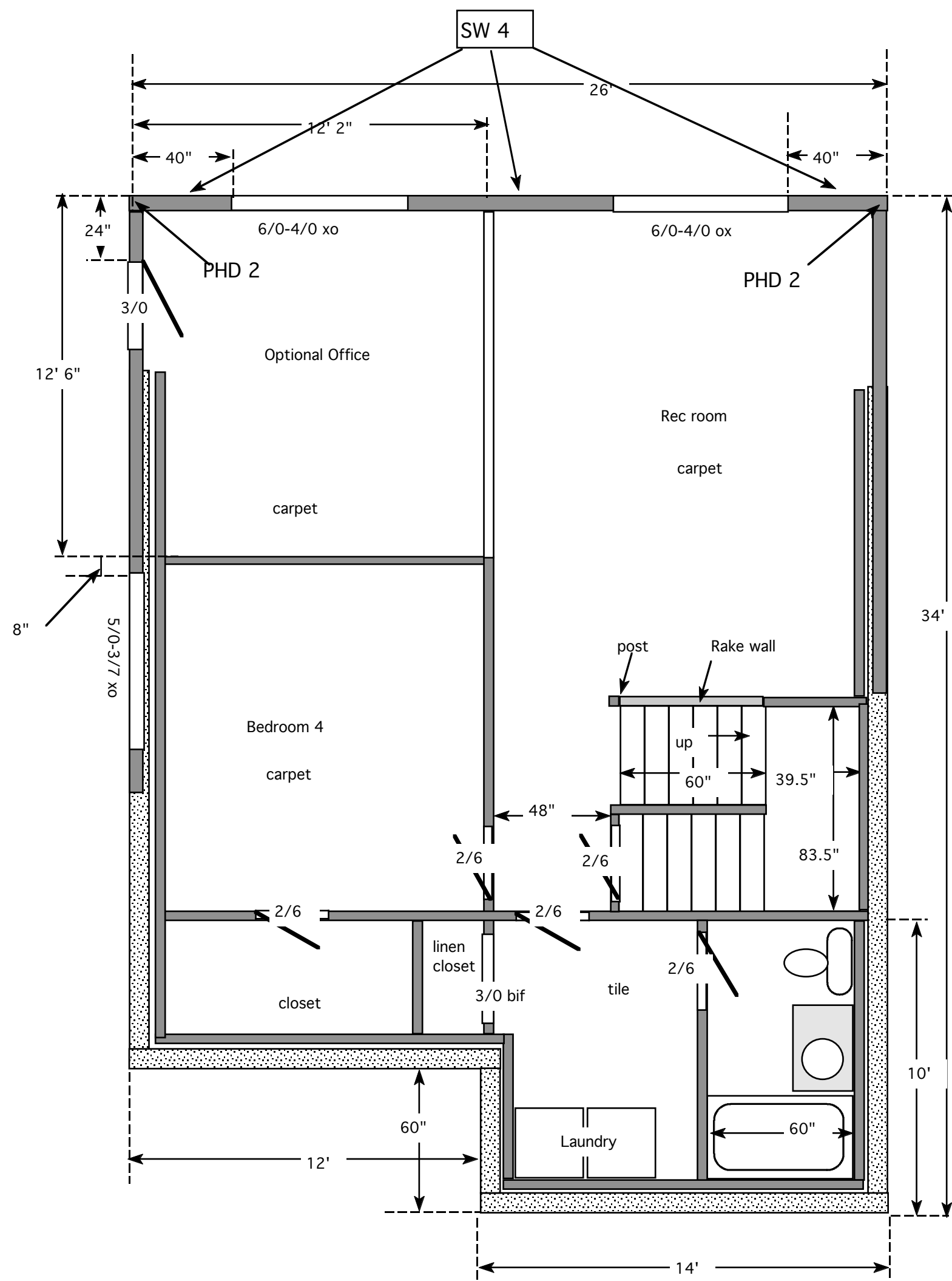
Finished Basement area = 850 sq. ft.
